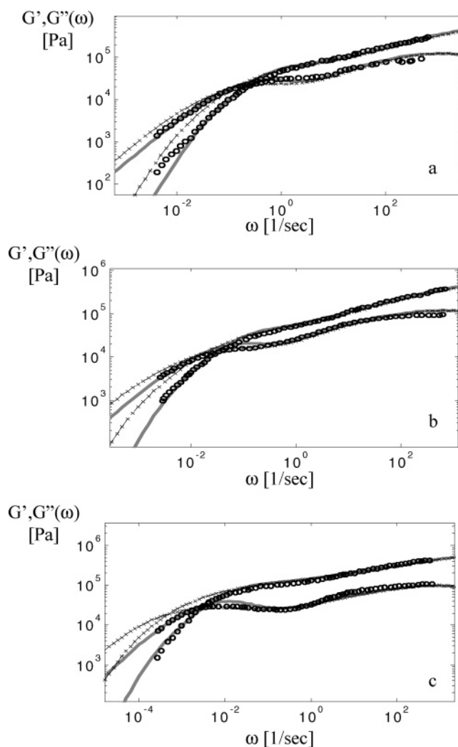
Figure 12. Storage and loss moduli of samples PB1 (a), PB2 (b), and PB4 (c), calculated without any reptation ( \times \times \times ), or with reptation, by considering that the “solvent” polymer fraction for the backbone is described by eqs 19 and 20 (---); see text for details.
