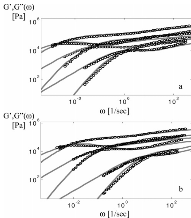
Figure 10. Linear viscoelastic moduli of samples PB8 (see Table 1) diluted in solvent at different concentrations: \Phi_{\text{polym}} = 1, 0.73 , and 0.5 (a); \Phi_{\text{polym}} = 0.9, 0.63 , and 0.34 (b). Comparison between predictions (---) and experimental (symbols) data.
