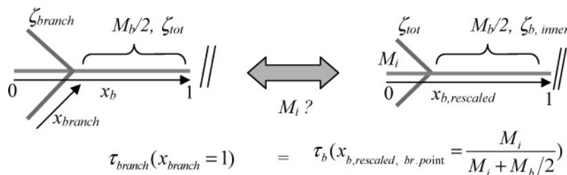
Figure 2. Definition of an “equivalent pom-pom molecule” used to calculate the fluctuations times of the segments localized in the inner part of the backbone.
