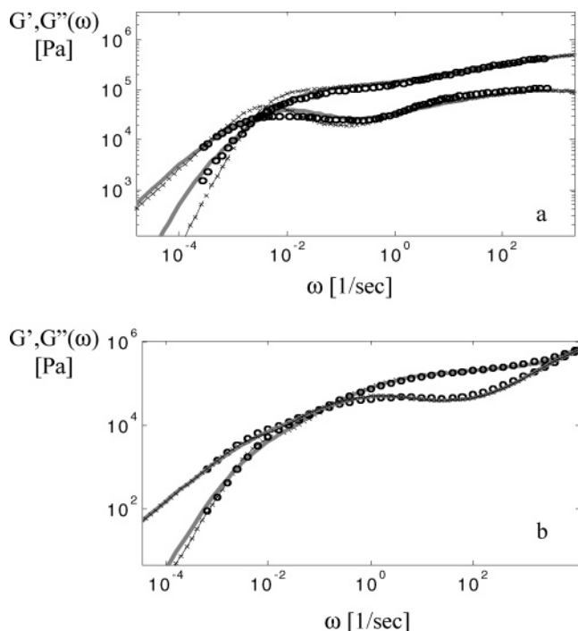
Figure 13. Storage and loss moduli of samples PB4 (a) and PS3 (b), calculated by considering a polydispersity of 1.05 (---), or by considering the samples as monodisperse ( \times \times \times ).
